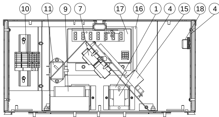
Remote Dispenser (Cut-away side view)
