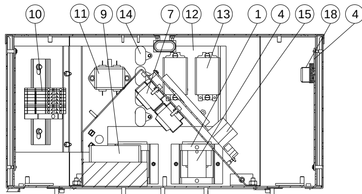
Suction Pump (Cut-away side view)
