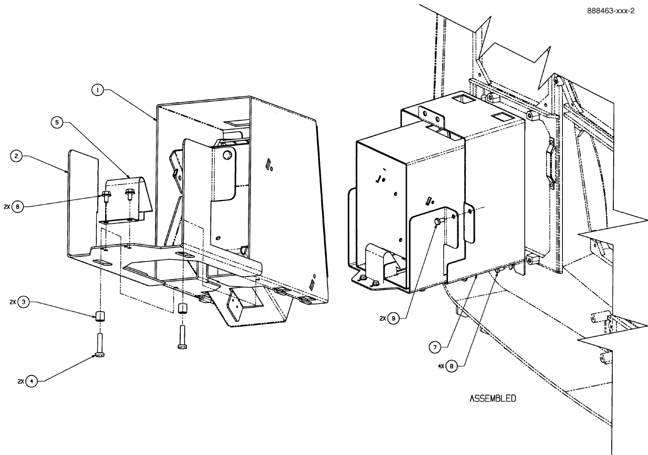
FIGURE 37. 888463-XXX - PRINTER ASSY, OVATION
