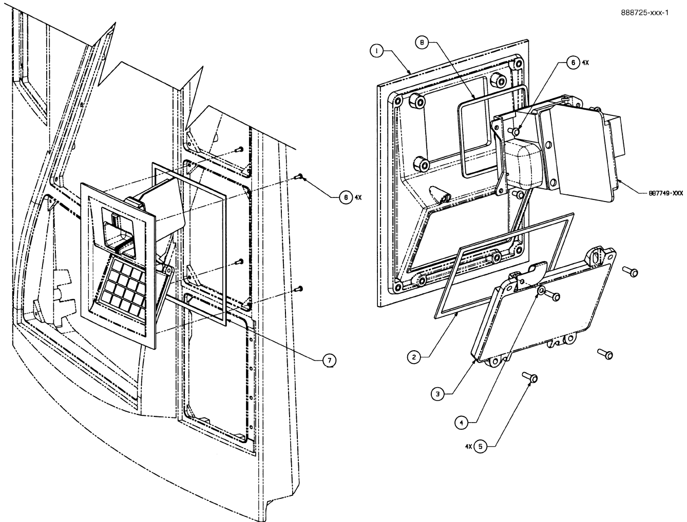
FIGURE 39. 888725-XXX - PANEL ASSY, CARD READER/KEYPAD
