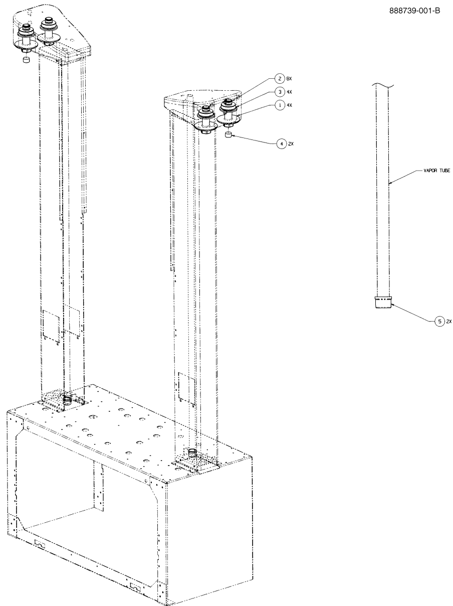
FIGURE 47. 888739-001 - OUTLET MODULE NON VAPOR, OVATION
