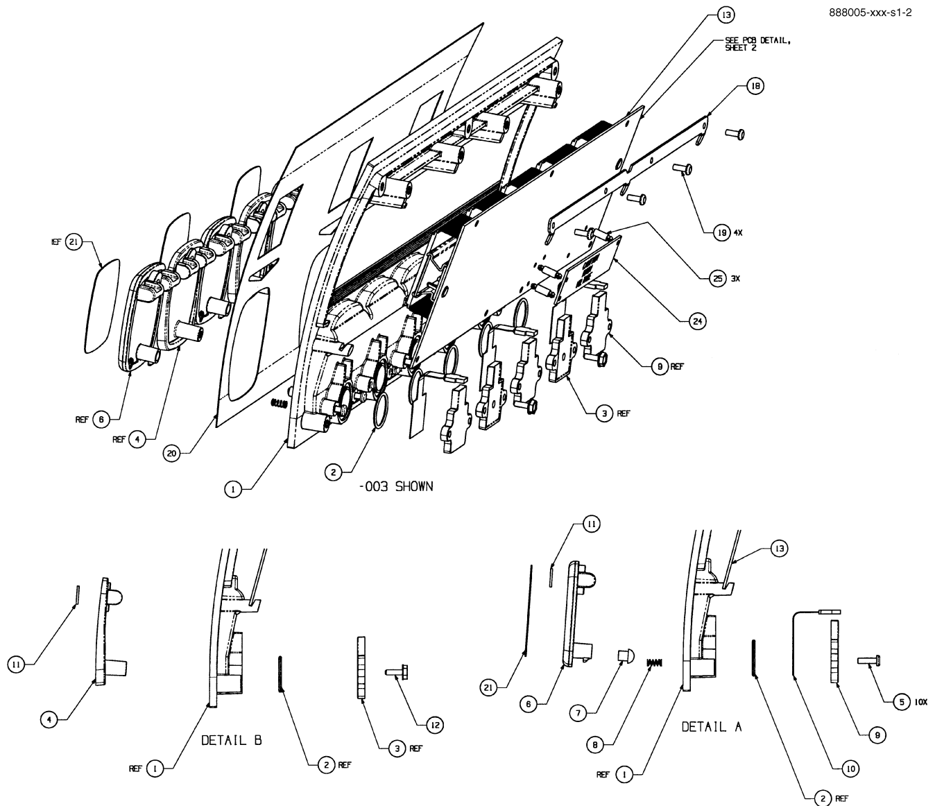
FIGURE 33. 888005-XXX-S1 - PANEL ASSY, PUSH TO START
