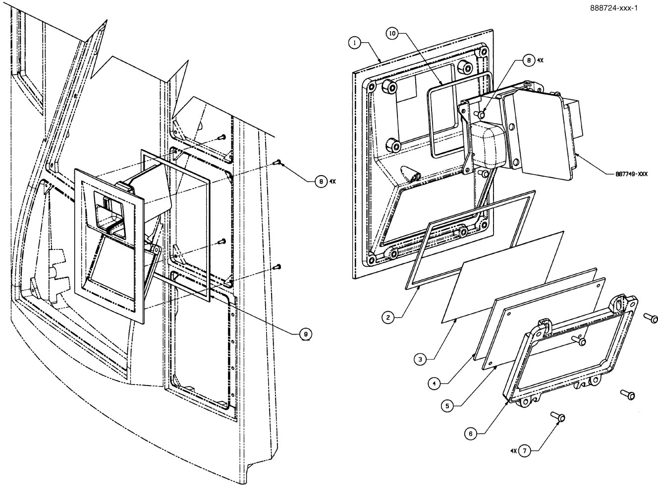
FIGURE 38. 888724-XXX - PANEL ASSY, CARD READER
