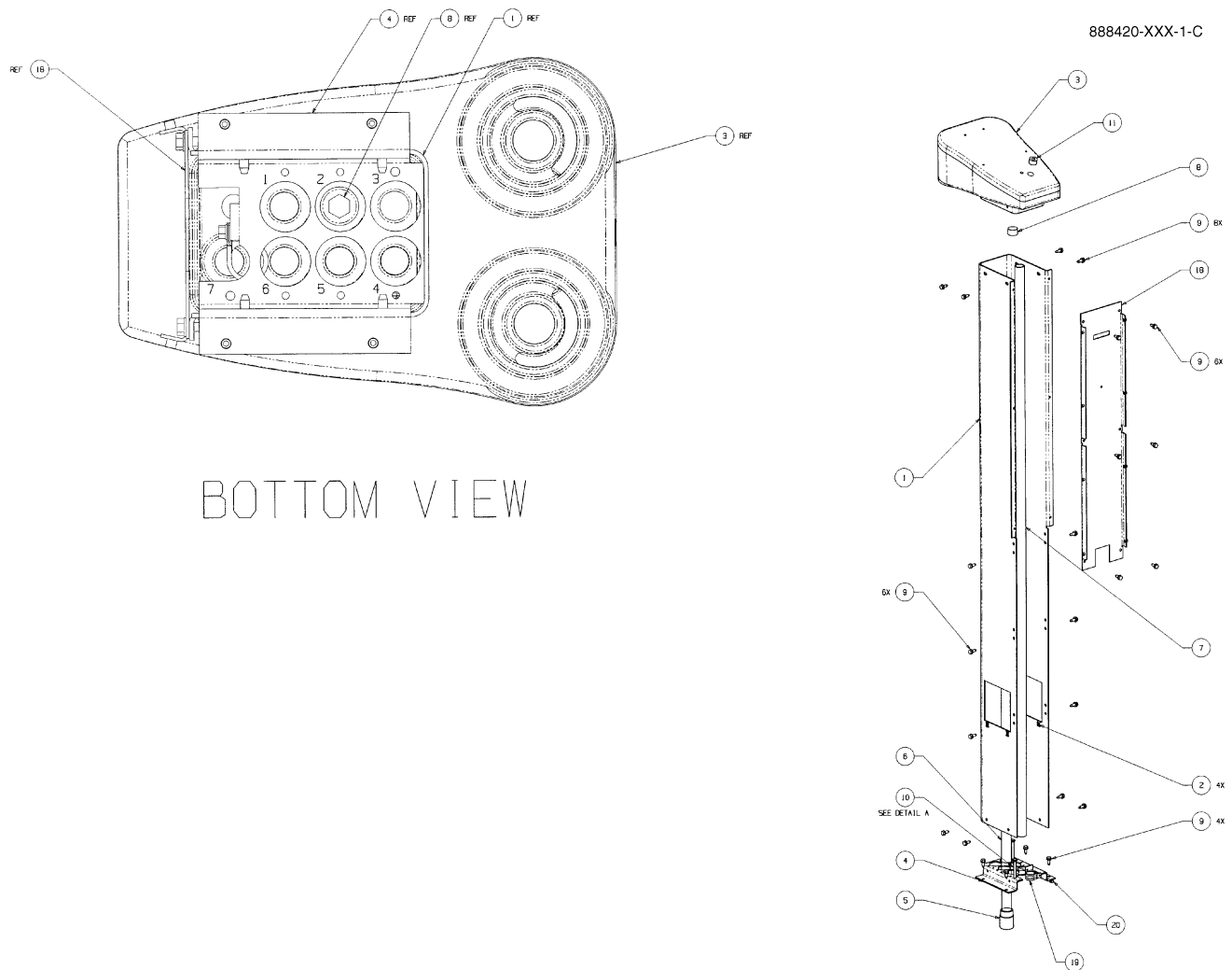
FIGURE 46. 888420-XXX-S1 - COLUMN ASSY, OVATION
