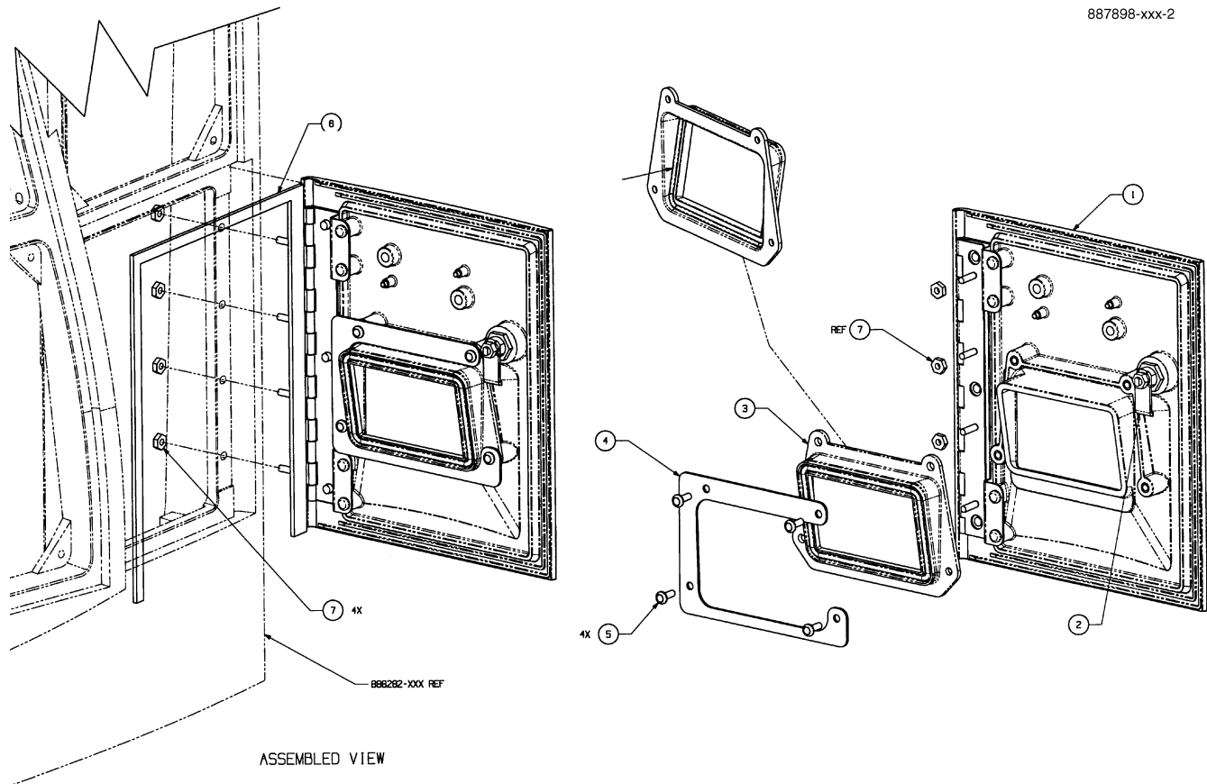
FIGURE 36. 887898-XXX - PRINTER DOOR ASSY
