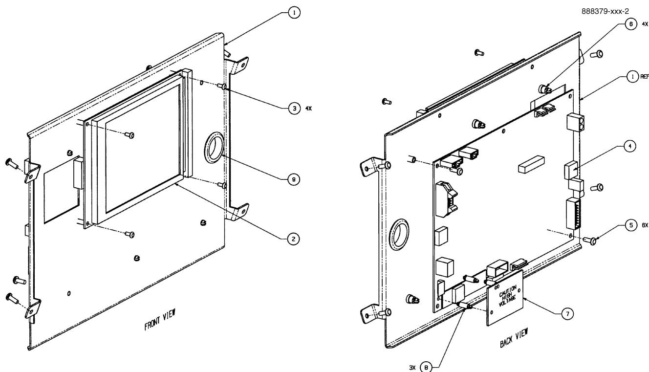
FIGURE 32. 888379-XXX - MOUNTING BRACKET ASSY, QVGA/BCB
