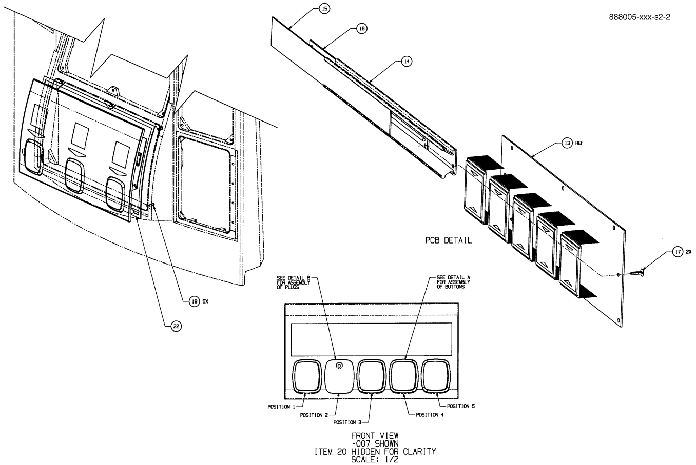
FIGURE 34. 888005-XXX-S2 - PANEL ASSY, PUSH TO START
