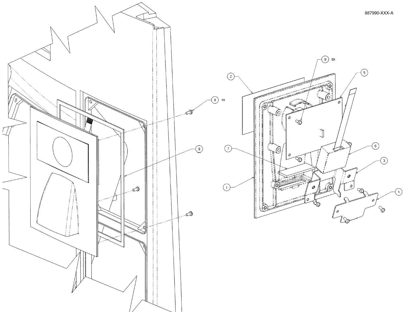
FIGURE 42. 887990-XXX - SCANNER PANEL ASSY
