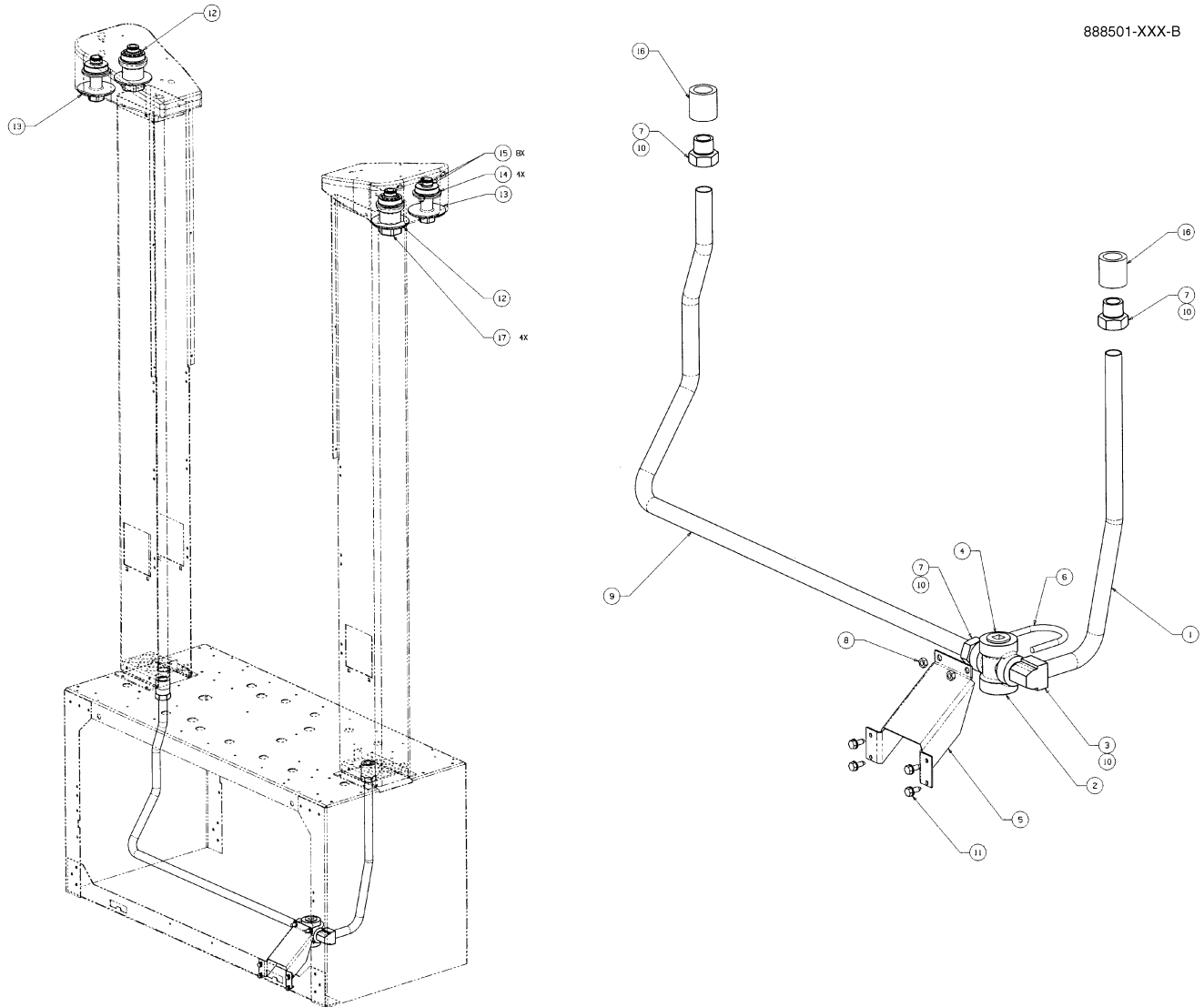
FIGURE 48. 888501-XXX - BALANCE VAPOR RECOVERY MODULE, OVATION
