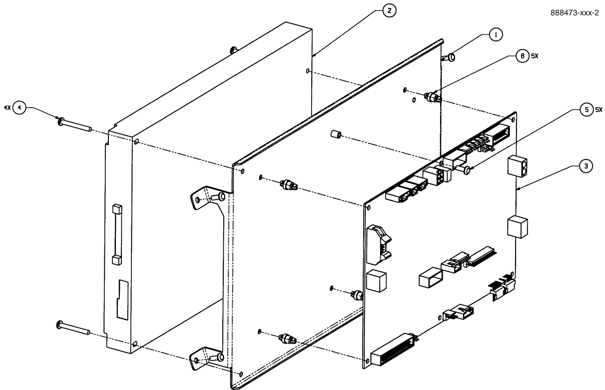
FIGURE 41. 888473-XXX - 10.4 VGA/BCB BRACKET ASSY
